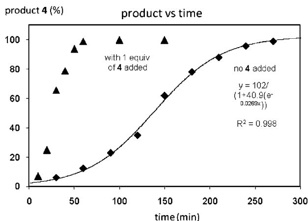
Figure 16. Kinetic data of C–F reductive elimination from 3 .
