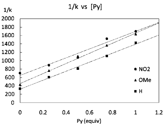
Figure 15. Rate dependence on pyridine concentration for the three 7-substituted benzo[ h ]quinolyl Pd(IV) pyridine complexes 2 , 10a , and 10g .
