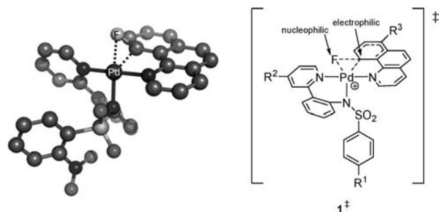
Figure 19. Computed transition state 1^\ddagger for reductive elimination from 1 and predicted transition state based on Hammett analysis.
