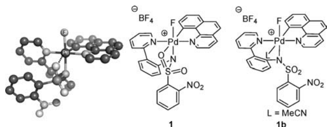
Figure 7. Energy minimized structure of 1 . The computed energy difference ( \Delta H_{298}^\ddagger ) between 1 and 1b is 2.2 \text{ kcal}\cdot\text{mol}^{-1} favoring 1 .
