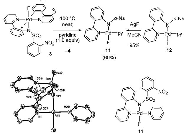
a ORTEP representation of Pd(II) fluoride complex 11 with ellipsoids drawn at 50% probability (hydrogen atoms omitted for clarity). Pd–F: 1.981 Å.
